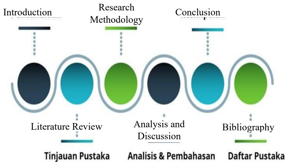
Fig. 1. Research Flow.
