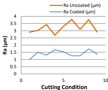
Fig. 4. Comparative graph of surface roughness (Ra)
