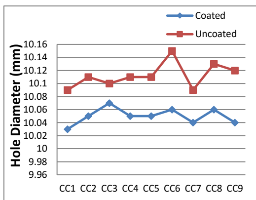
Fig.6. Diameter Error
