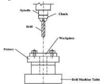
Fig. 3. Drilling Machine
