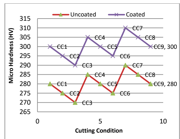
Fig. 9. Micro Hardness
