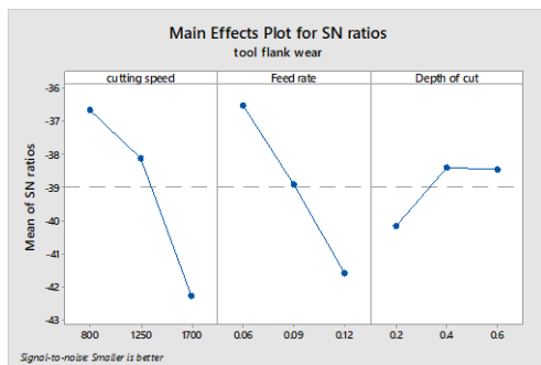
Figure 8, Mean S/N ratio of tool flank wear
