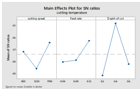
Figure 4. Mean S/N ratio of cutting temperature
