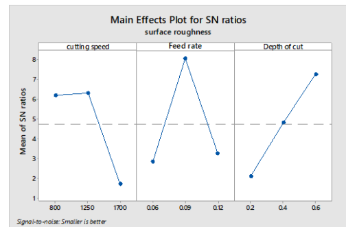
Figure 6. Mean S/N ratio of surface roughness
